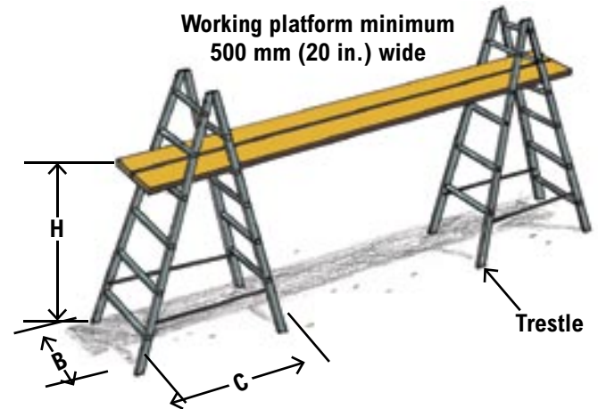
This is an example of a trestle scaffold.
