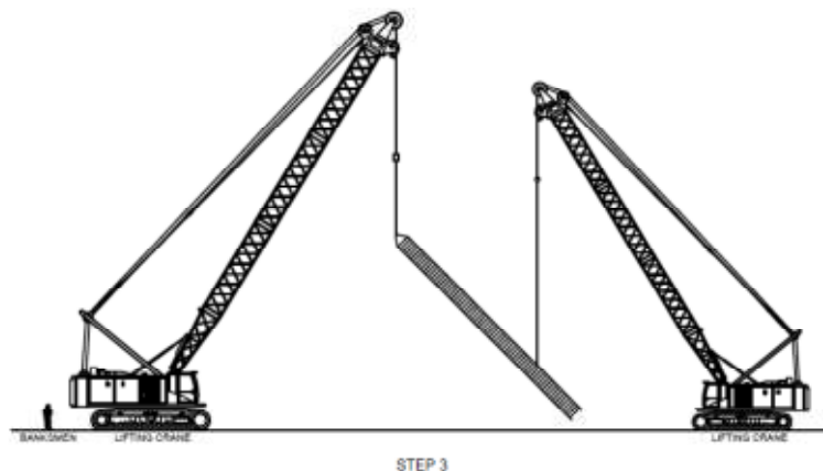
Figure 2: Two point lifting
