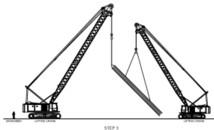
Figure 1: Three (3) point lifting
